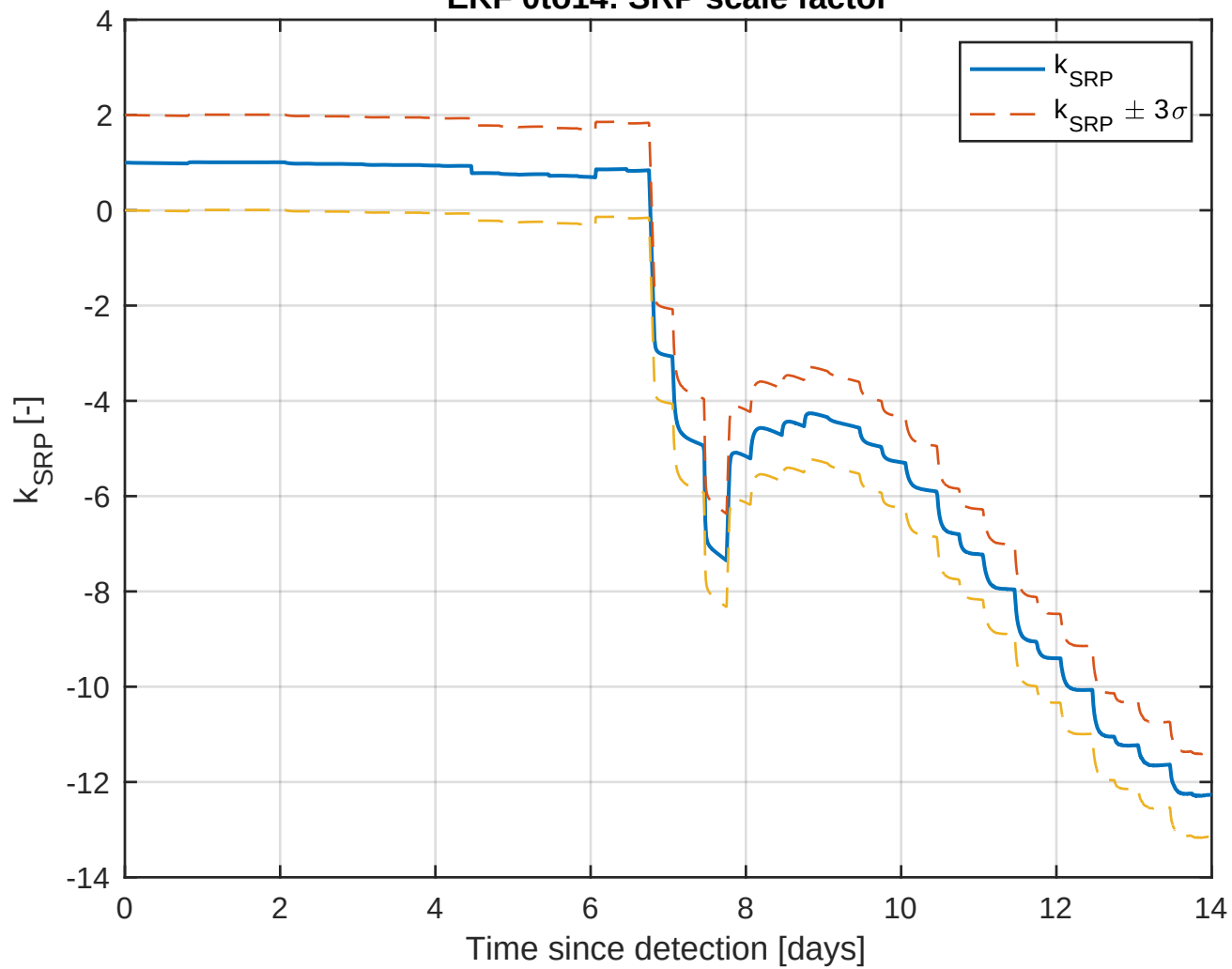
EKF 0to14: SRP scale factor
